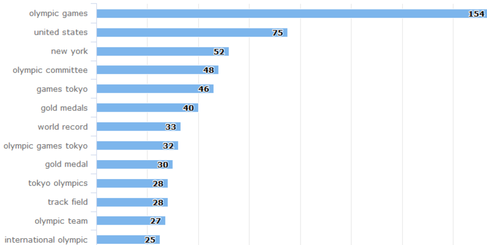
Term Frequency
